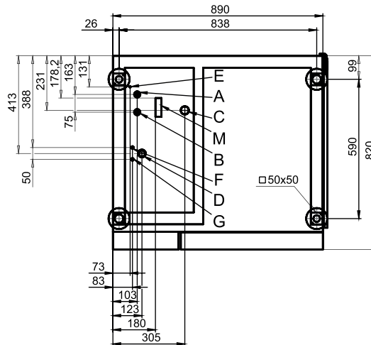
Connection points
